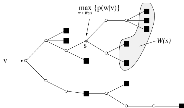
Figure 1: Illustration of LM tree factorization.
